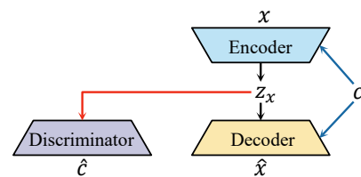
Figure 1: An illustration of domain adversarial training over a conditional generation architecture.
