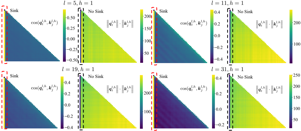
Figure 15: Cosine similarity and \ell_2 -norm product between keys and queries in LLaMA3-8B Base.
