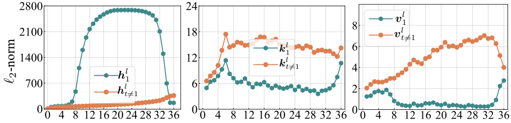
Figure 11: \ell_2 -norm of hidden states/keys/values of the first token/other tokens in GPT2-Large.
