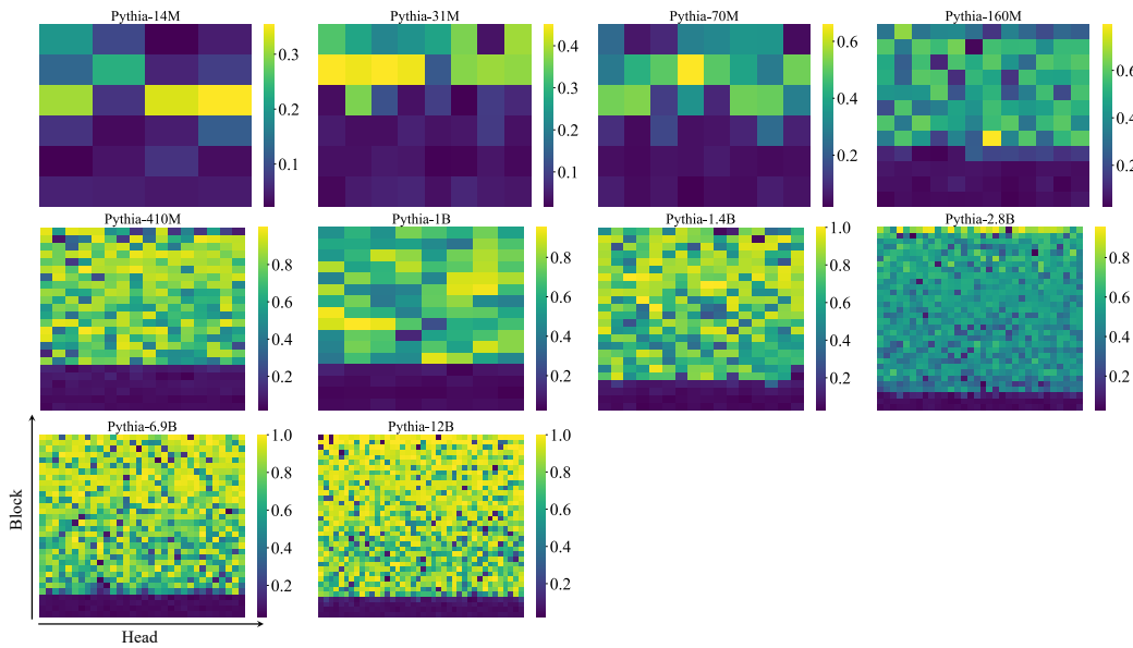
Figure 23: Distribution of importance scores for the first token across different blocks and heads in the Pythia family.
