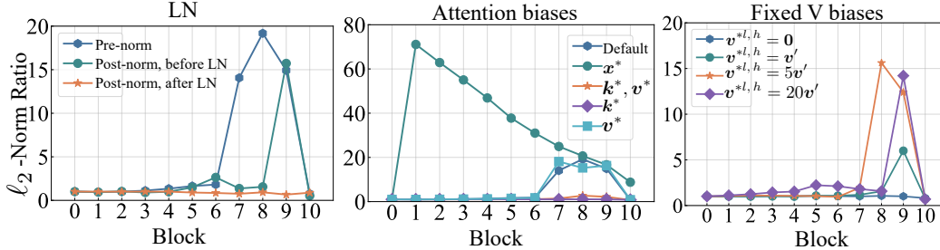
Figure 7: \ell_2 -norm ratio of h_1^l and mean of h_{l \neq 0}^l . (Left) Massive activations exist not in hidden states in post-norm LMs, but in the features before LN. (Middle) LMs with KV biases or K biases have no massive activations, while LMs with a learnable sink token or V biases have massive activations. (Right) Massive activations emerge when increasing the \ell_2 -norm of fixed v^{*l,h} for the setup of K biases.
