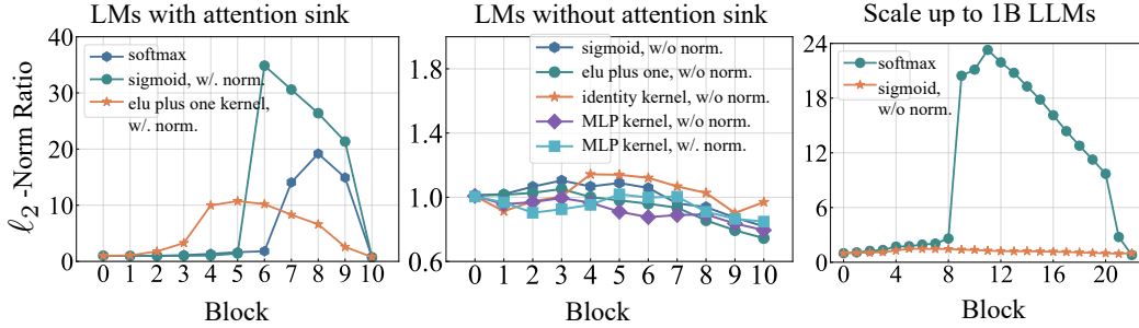
Figure 8: We visualize the \ell_2 -norm ratio of \mathbf{h}_1^l and mean of \mathbf{h}_{t \neq 0}^l . (Left) Massive activations exist in LMs with attention scores that are non-negative and added up to one. (Middle) Massive activations do not exist in LMs with independent attention scores. (Right) When scaling the model size to 1B, LLMs with sigmoid attention (no normalization) still have no massive activations.
