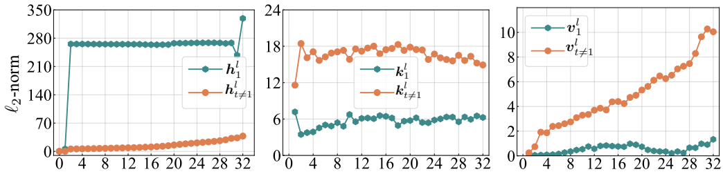
Figure 12: \ell_2 -norm of hidden states/keys/values of the first token/other tokens in Mistral-7B.
