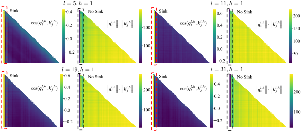
Figure 16: Cosine similarity and \ell_2 -norm product between keys and queries in LLaMA2-7B Base.
