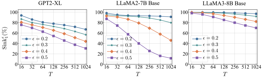
Figure 3: The metric \text{Sink}_1^\epsilon (averaged on 100 sequences) tends to decrease with larger token lengths T . This tendency becomes more obvious with the more strict definition of attention sink (larger \epsilon ).
