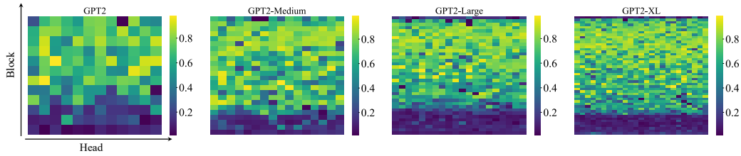
Figure 22: Distribution of importance scores for the first token across different blocks and heads in the GPT2 family.
