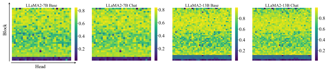
Figure 18: Cosine similarity and \ell_2 -norm product between keys and queries in GPT2-Large.
