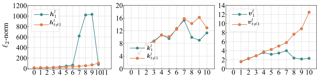
Figure 14: \ell_2 -norm of hidden states/keys/values of the first token/other tokens in our small LLaMA model.
