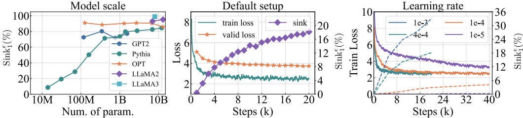
Figure 4: (Left) Attention sink emerges in small LMs. (Middle) Dynamics of train/valid loss and Sink 1 ϵ during LM pre-training under the default setup. Attention sink emerges after certain optimization steps. (Right) Training loss (solid lines)/attention sink (dashed lines) dynamics of LMs using different learning rates. We observe that with smaller learning rates, attention sink tends to emerge after more optimization steps and be less obvious.
