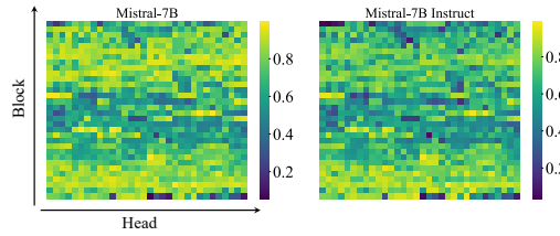
Figure 21: Distribution of importance scores for the first token across different blocks and heads in the Mistral family.
