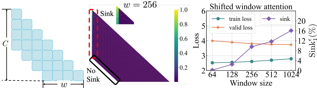
Figure 6: (Left) Shifted window attention pattern. (Middle) In LMs with window attention, attention sink appears on the first token, but not on the “first token” within each window. (Right) Attention sink tends to emerge when the window size is large enough.
