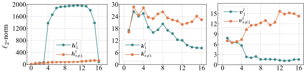
Figure 13: \ell_2 -norm of hidden states/keys/values of the first token/other tokens in Pythia-1B.
