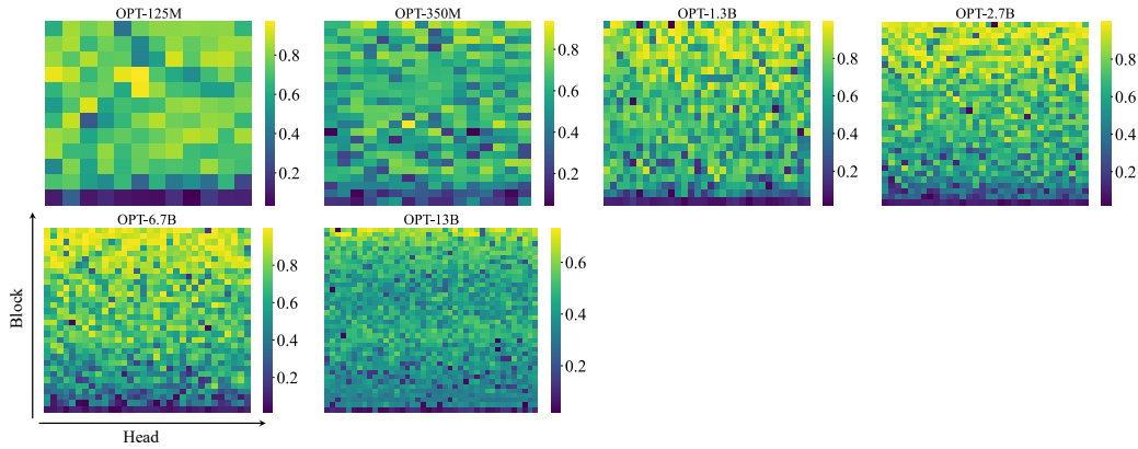
Figure 24: Distribution of importance scores for the first token across different blocks and heads in the OPT family.
