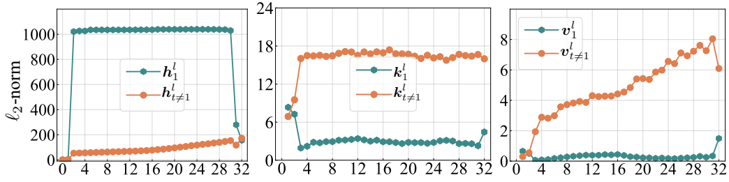
Figure 10: \ell_2 -norm of hidden states/keys/values of the first token/other tokens in LLaMA2-7B Base.
